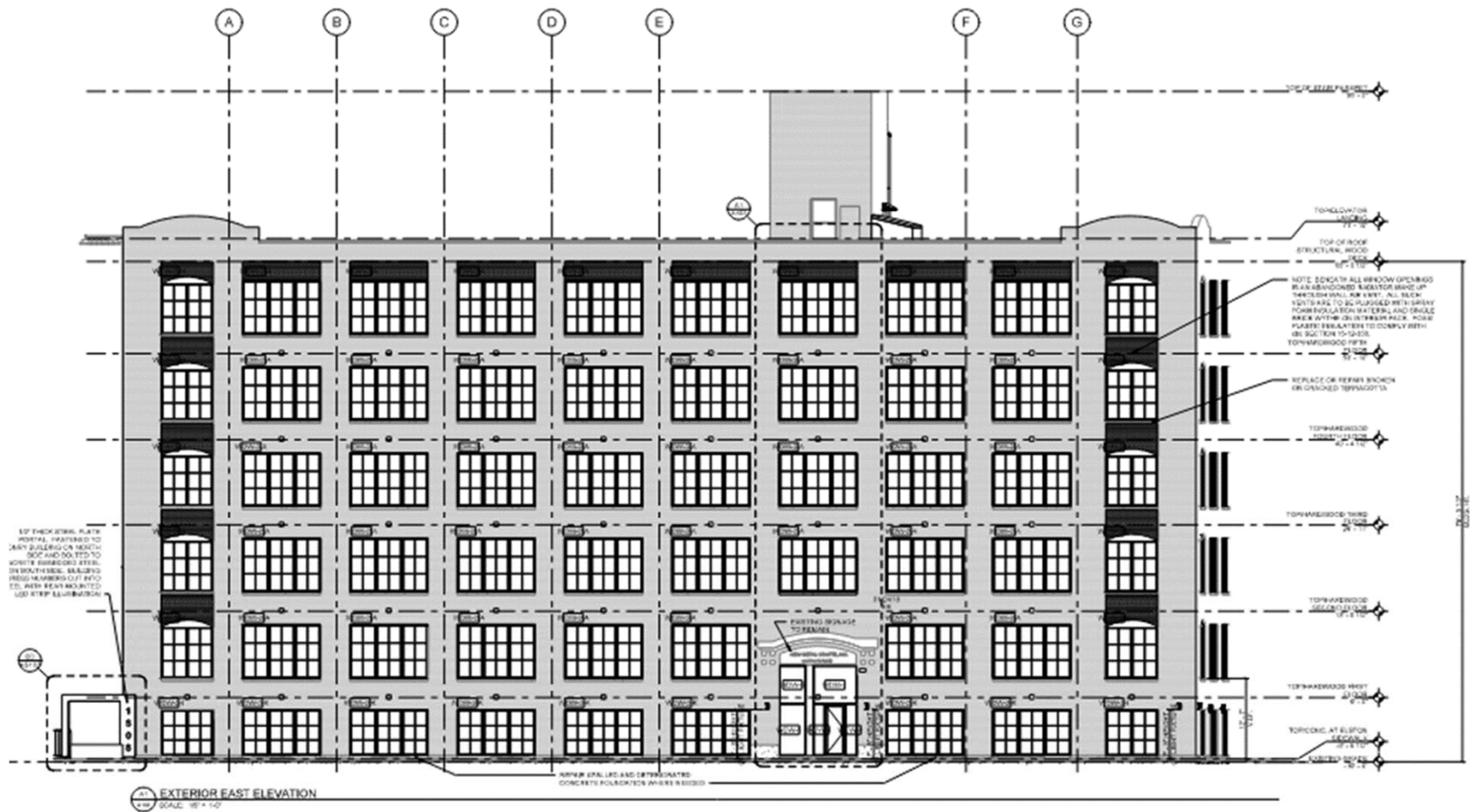
BUILDING ELEVATION (EAST ELEVATION)
