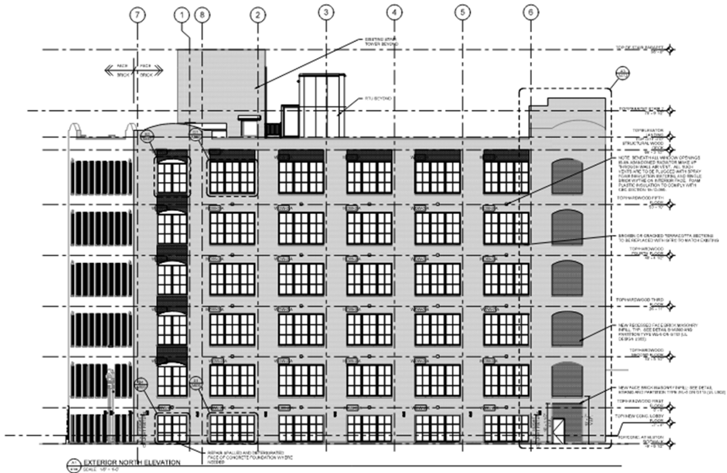
BUILDING ELEVATION (NORTH ELEVATION)
