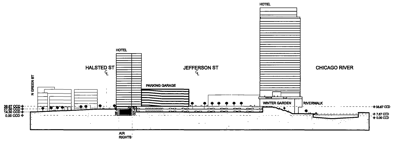
SITE SECTION AA' LOOKING NORTH
